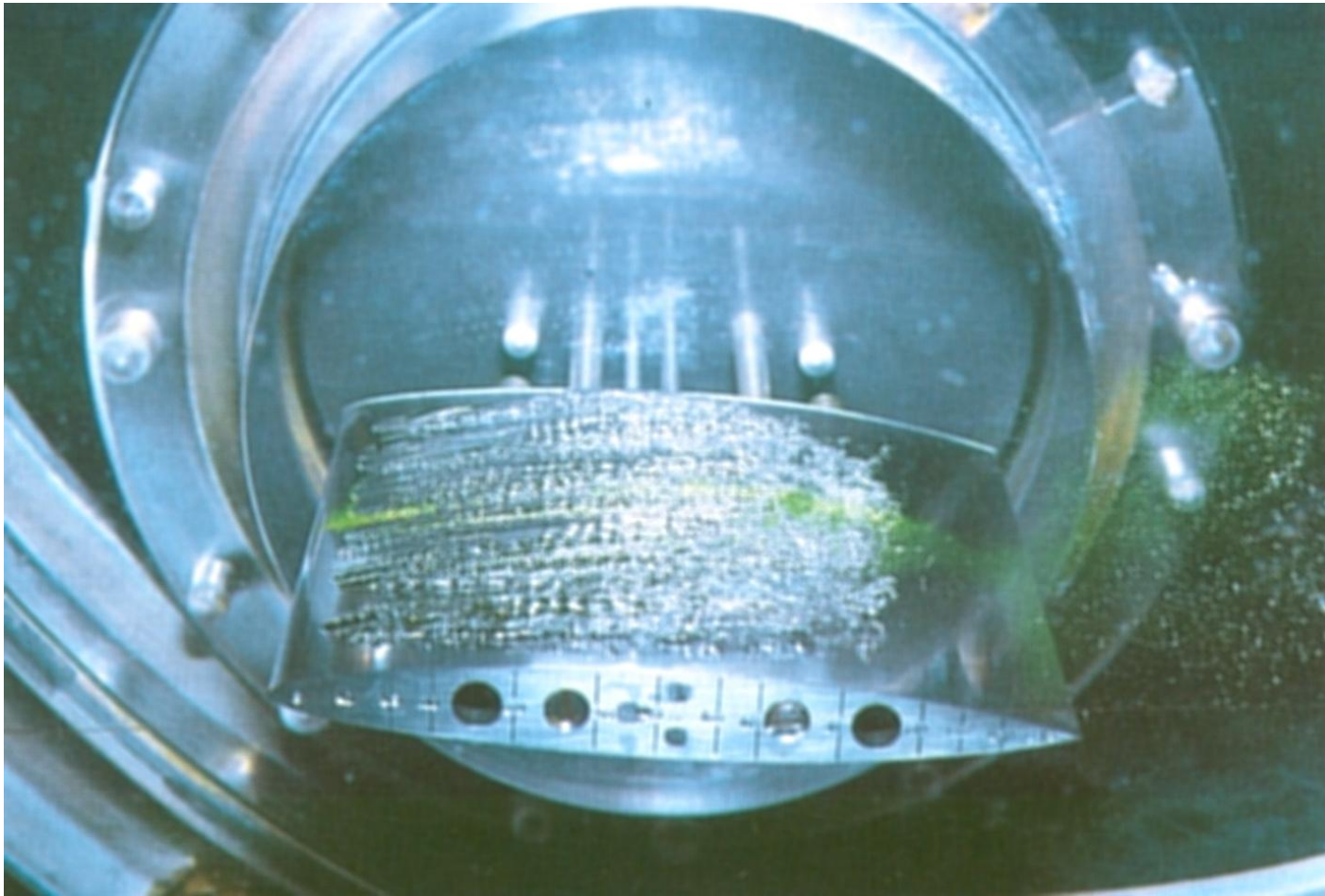
Schichtkavitation
