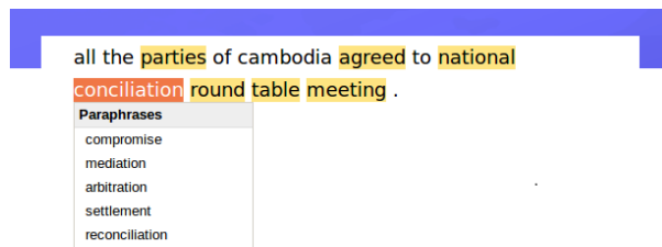
Figure 1: An online interface for the semantic writing aid application. Paraphrase suggestions are presented from a systematic combination of different NLP resources.
