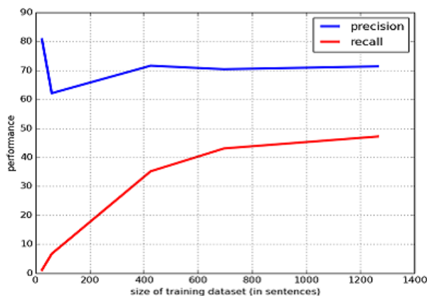
Figure 2: Learning curve showing the performance of interactive automation using different sizes of training data
