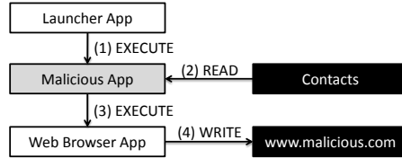
Fig. 1. Example confused deputy attack, where a malicious app deputizes the web browser to exfiltrate sensitive contacts information.
