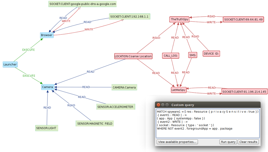
Fig. 4. Screenshots of the DroidAuditor client while analyzing malicious spyware applications. Subgraphs matching the displayed query are highlighted in red.
